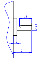
Detailed dimensions of gearbox output spindle
