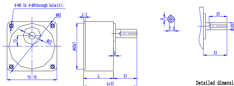
Detailed dimensions of gearbox output spindle
